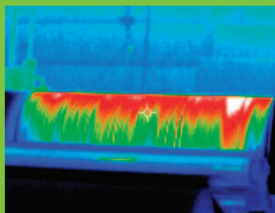
This thermal image highlights uneven cooling on a cooled paper roller.
